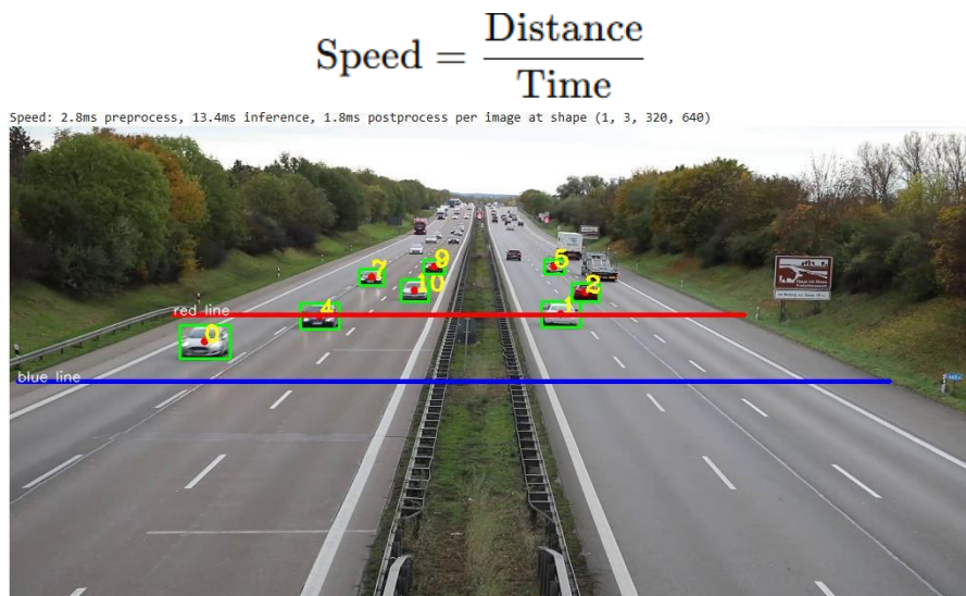
Figure 1: Tracking of vehicles using YOLOv8 and centroid based tracking algorithm
